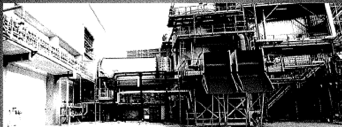
Incinerator Kiln \varnothing 4,7 x 14 m - Filago / Italy
