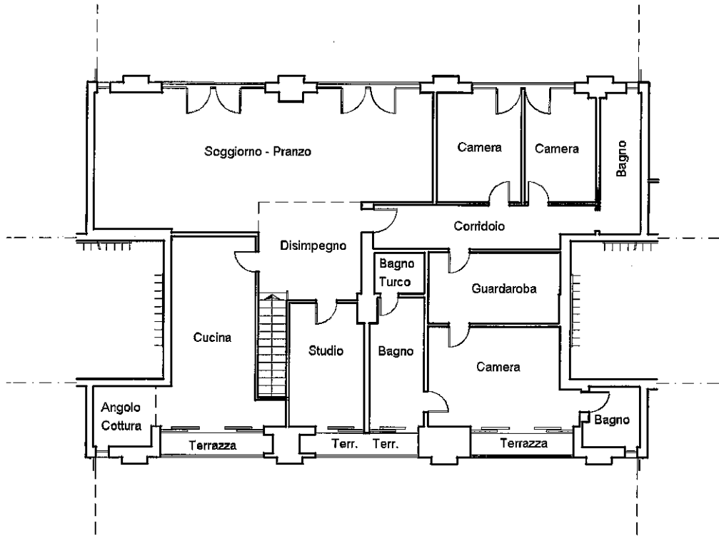
Piano Terzo, H = 2,70 m
