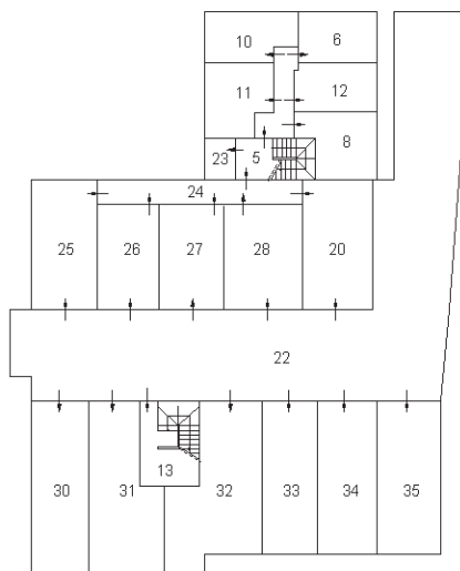
PIANO INTERRATO
