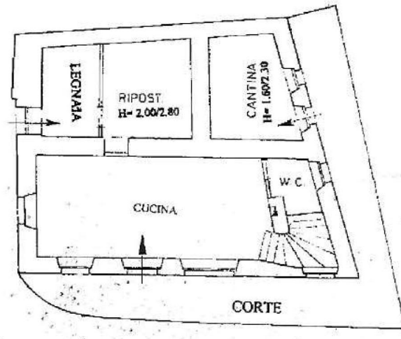
PIANO TERRA H = 2.65
