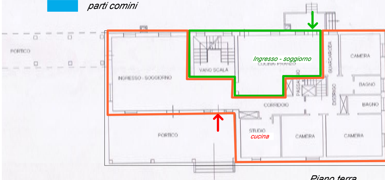
Piano terra
